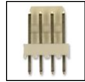
HEADER, SQUARE PIN, 2.54MM, 4WAY MOLEX 22-27-2041..
